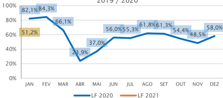
LOAD FACTOR 2019 / 2020
